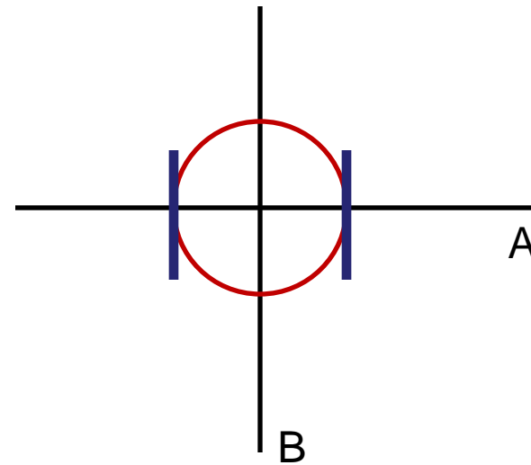
Orthogonal Design
